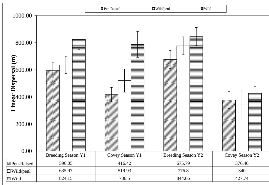
Figure 6: Linear dispersal distances (meters) for treatment groups on Groton Plantation, Allendale, SC during two seasonal groups (overwinter and breeding season) for both study years. Error bars represent the standard error of the treatment mean.
