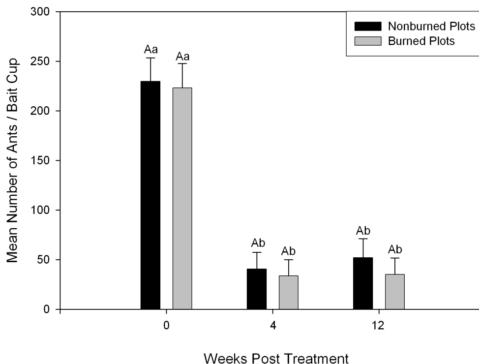
Figure 5: Mean ( \pm SE) number of foraging RIFA collected in bait cups from burned and nonburned plots in Calhoun County, Texas, in 2003. Means within a sampling time followed by the same upper case letter are not significantly different ( P > 0.05 ). Means within a burning treatment followed by the same lower case letter are not significantly different ( P > 0.05 ).
