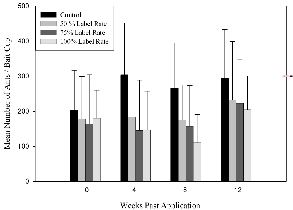
Figure 4: Mean ( \pm SE) number of foraging RIFA collected in bait cups for each insecticide treatment within four different sampling periods. Dashed line indicates threshold level of 300 foraging ants. Ants collected from plots in Goliad and Victoria Counties, Texas, in 2002.
